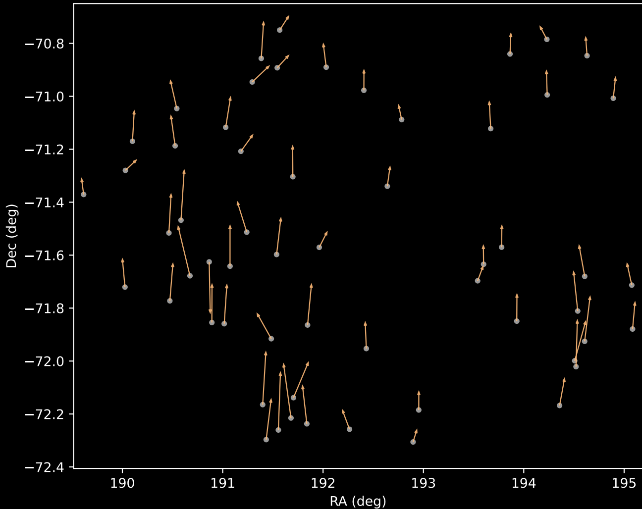
APOGEE DR17 Cluster 3 Proper Motion Vectors (n=58)
